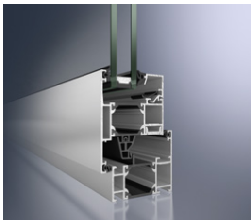
旭格AWS 65窗系统，外开 Schüco Window AWS 65, outward-opening
