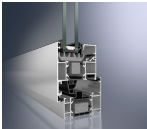
旭格AWS 70.HI窗系统，外开 Schüco Window AWS 70.HI, outward-opening
